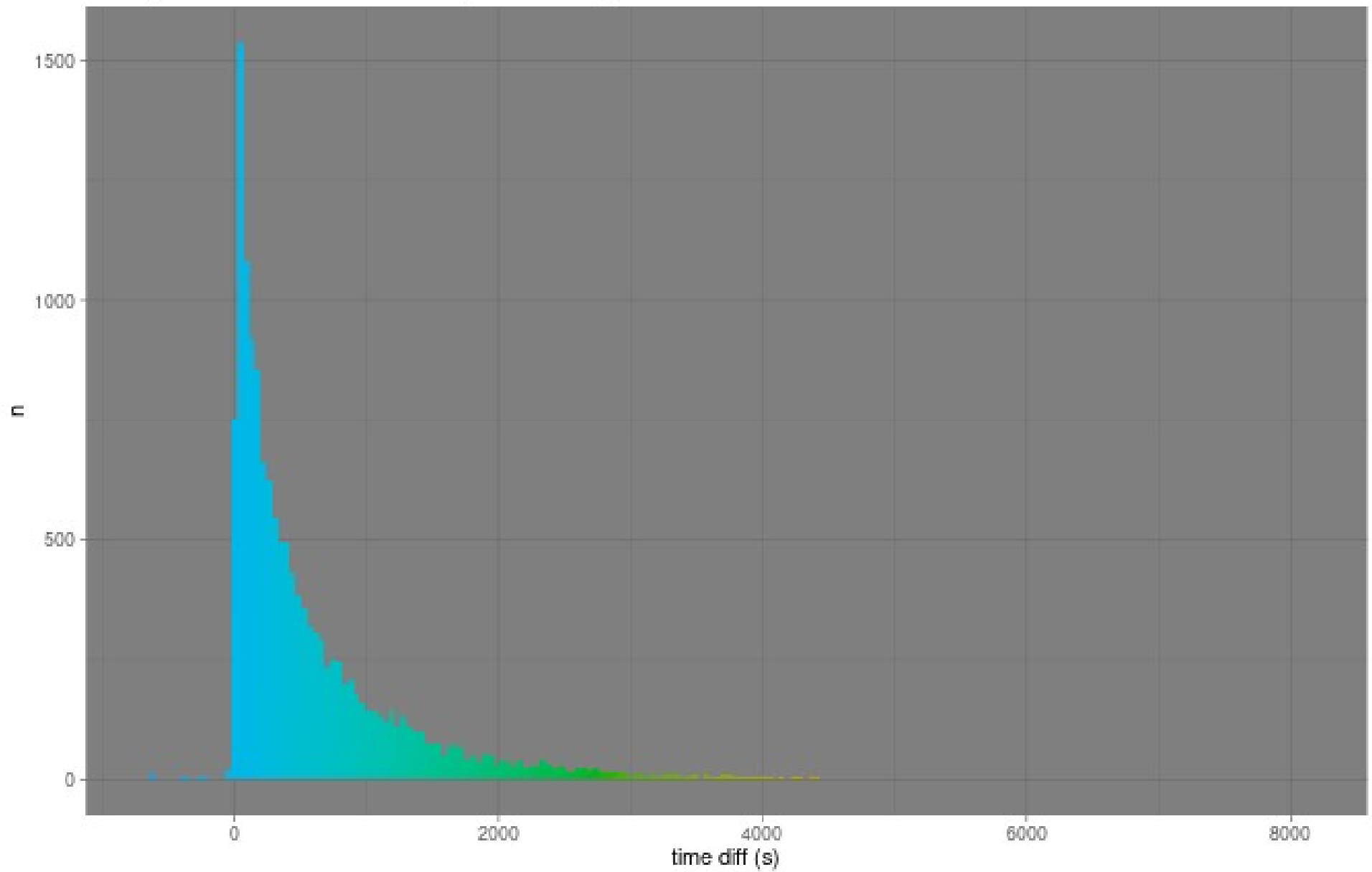
Histogram of block time deltas (ASERT era)
